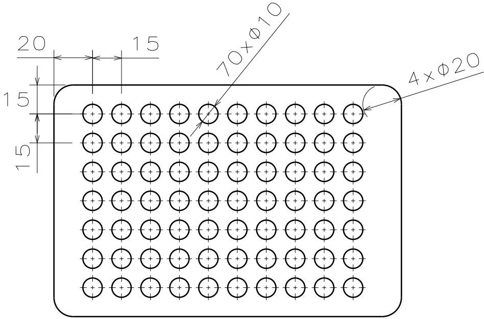
Front view Scale: 1:2
