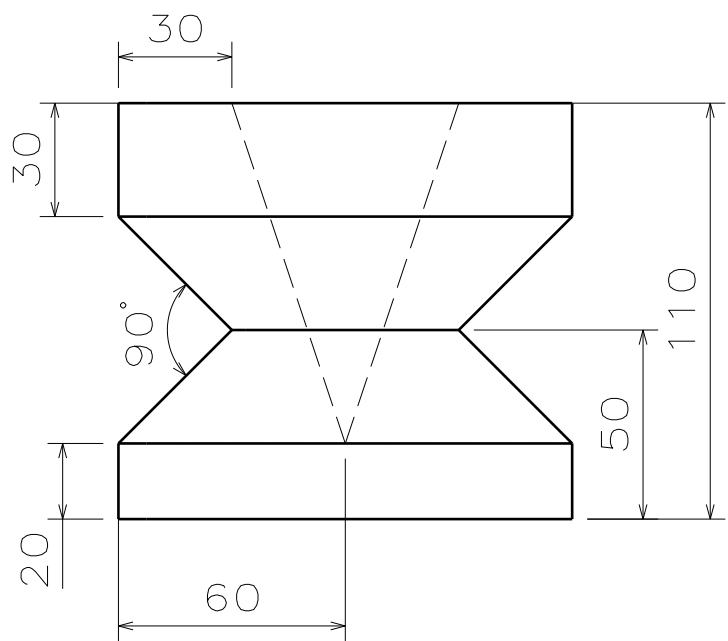
Front view Scale: 1:2
